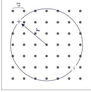
Mott-Wannier
